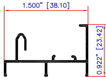
JAMBA LATERAL 1516
